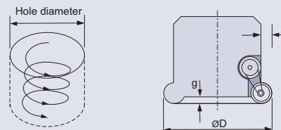
Helical milling
