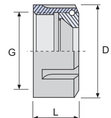
FORM E BALL BEARING NUT KUGELLAGER-MUTTER
